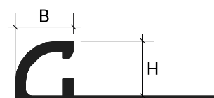
Synthetic Resin B = H + 1 \text{ mm}
